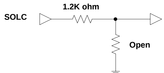
Figure6.SOLC input circuit is as below
