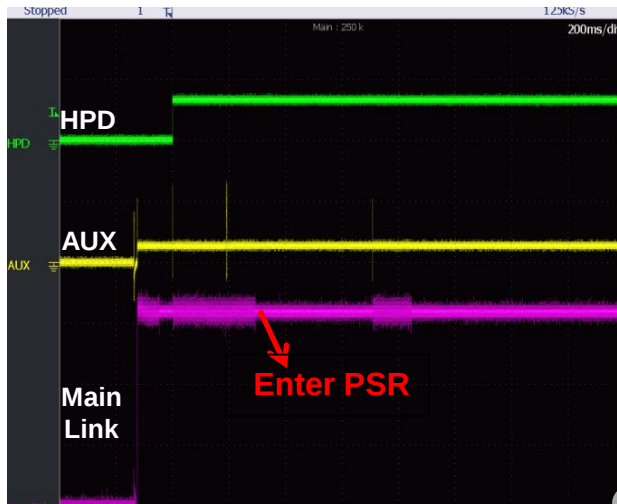
< Issue waveform >
