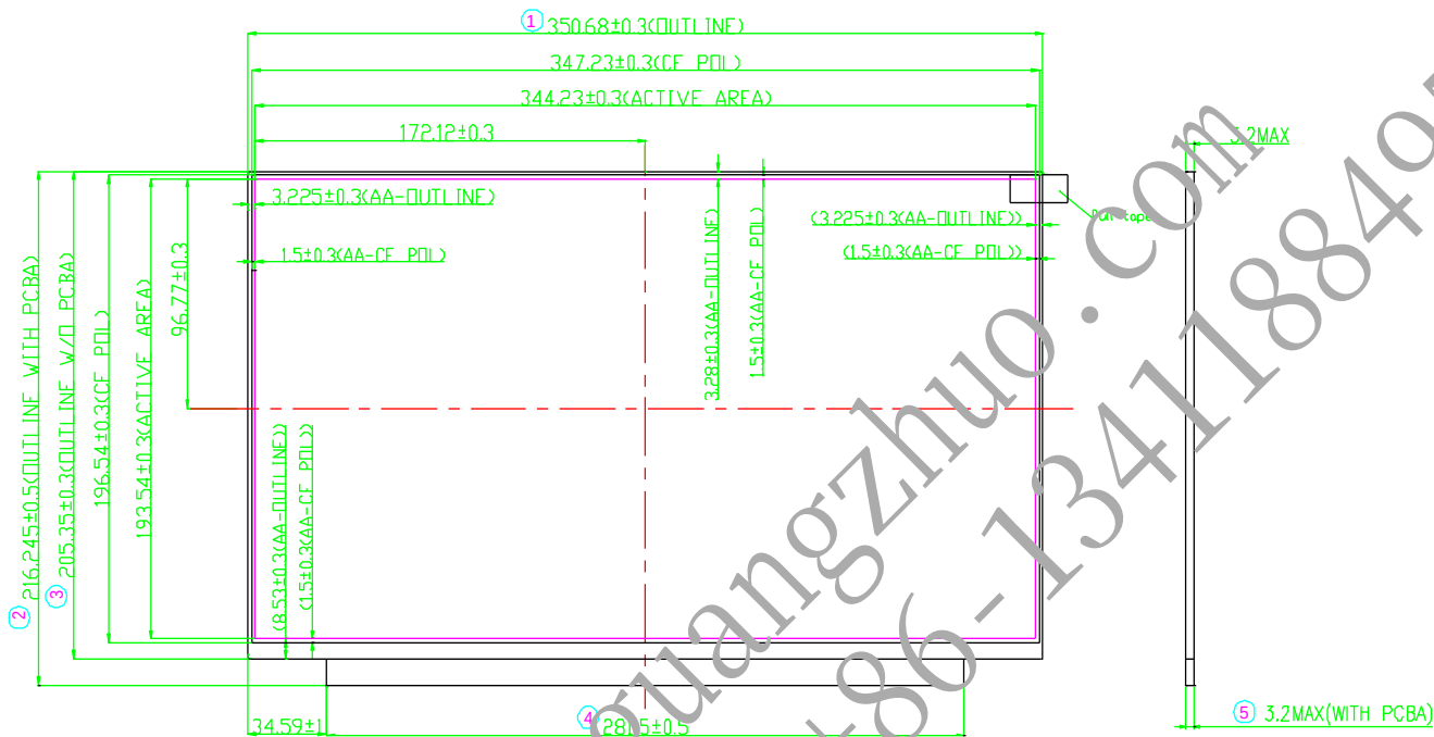
Figure 21. TFT-LCD Module Outline Dimension (Front View)
