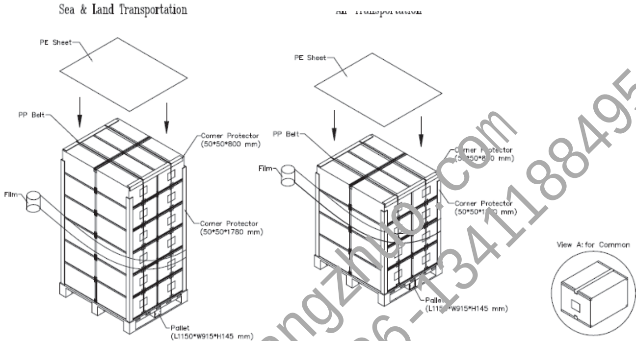
Figure. 7-3 Packing method
