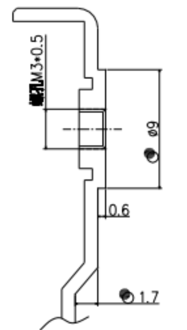
SECTION A-A (Scale: 5/1) Total 11pcs "a"
