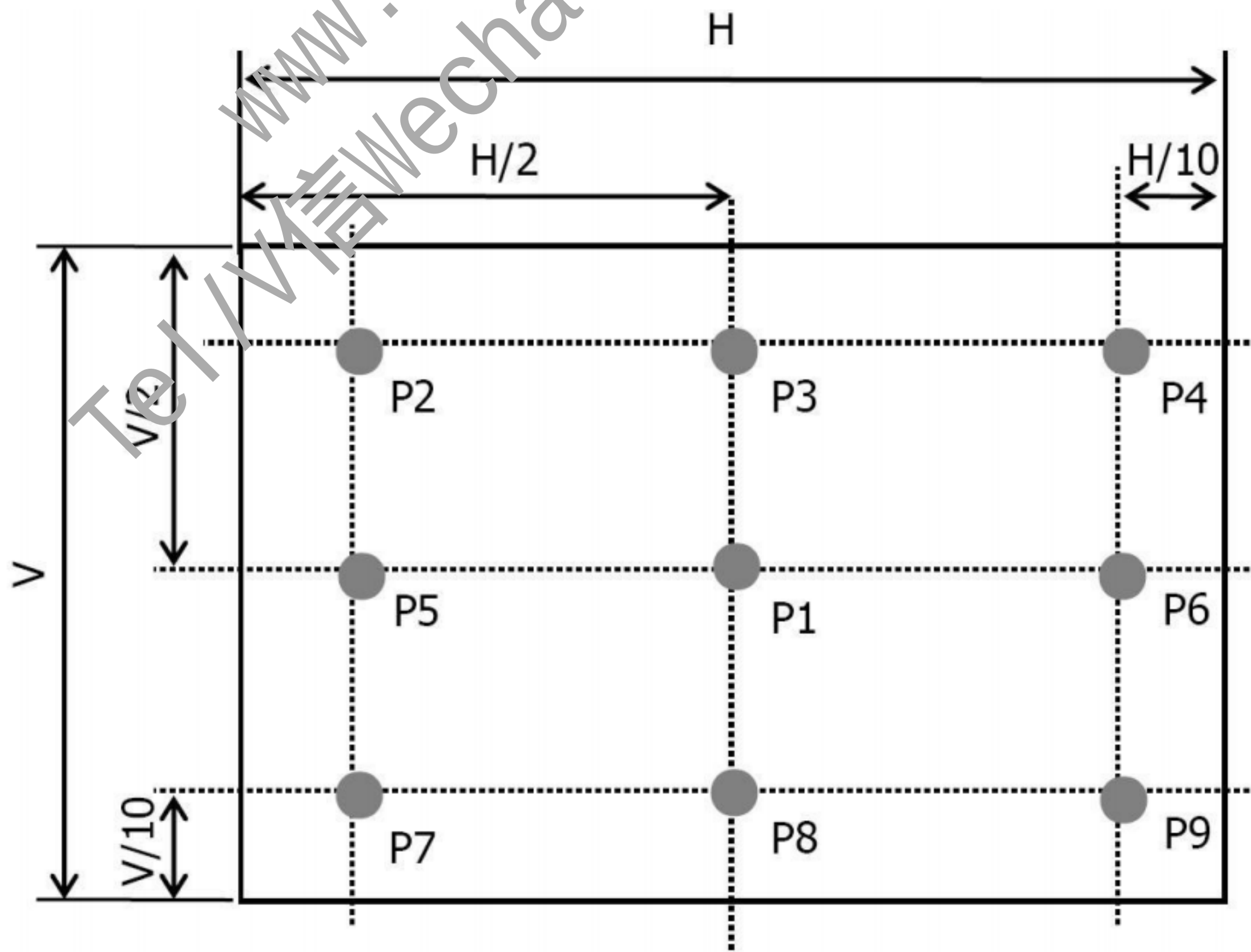
Figure 2. White Luminance and Uniformity Measurement Locations (9 points)
