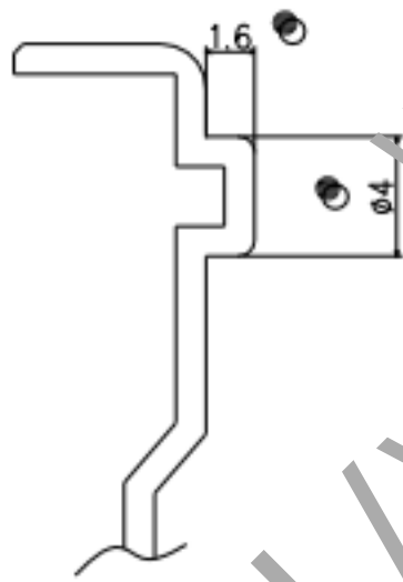
Section B-B(S:5/1) Total 4pcs "b"
