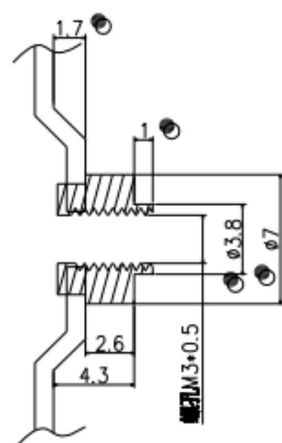
Section B-B(S:5/1) Total 4pcs "b"
