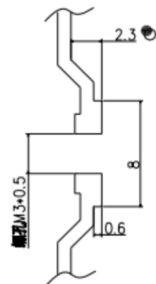
Section C-C(S:5/1) Total 4pcs "c"
