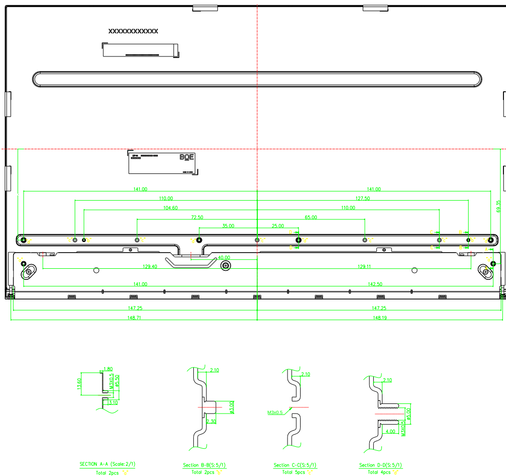
Figure 6. TFT-LCD Module Outline Dimensions (Back)
