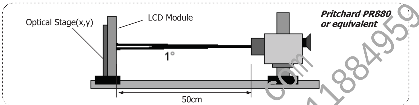
FIG.4-1 Optical Characteristic Measurement Equipment And Method
