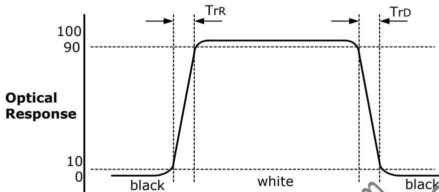
FIG.9 Response time
