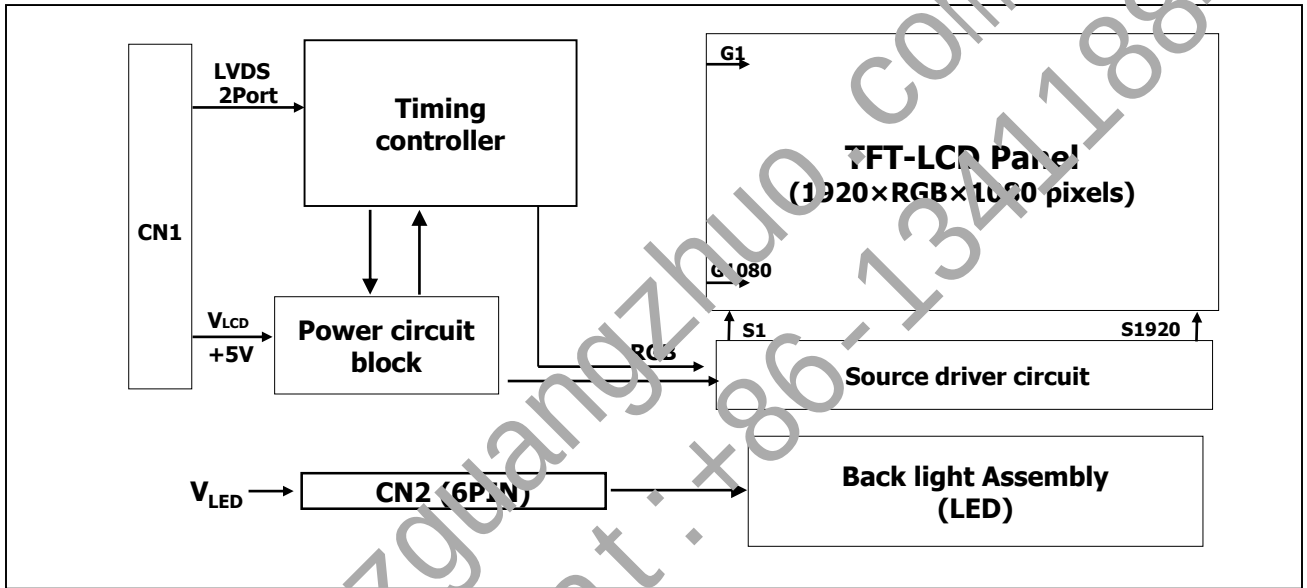
FIG.1 Block Diagram
