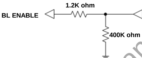
Figure5.DBC input circuit is as below
