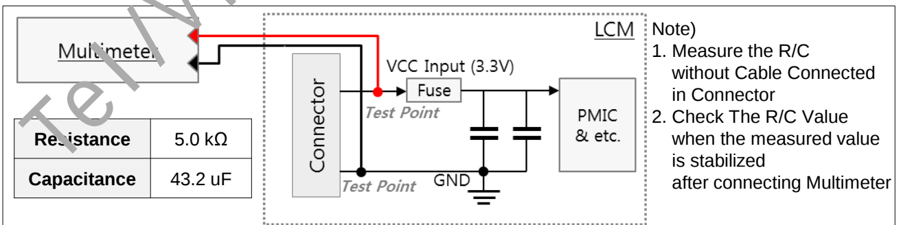
Figure7.Schematic Diagram for VCC Loop R/C Loading Measurement
