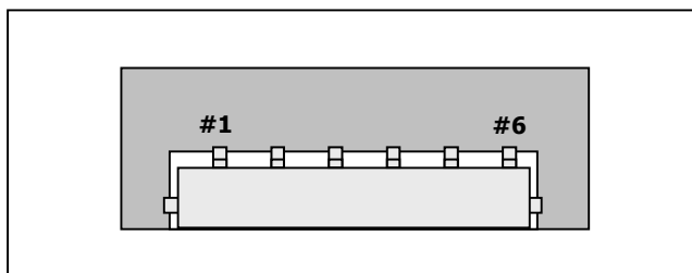
DF14A-6P-1.25H
