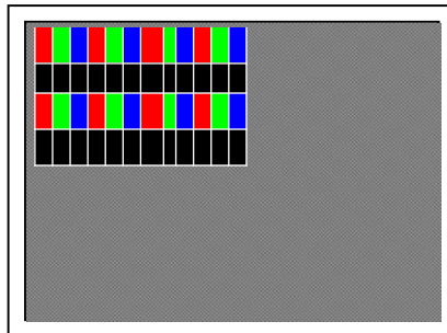
Maximum power pattern (Horizontal 1 by 1)
