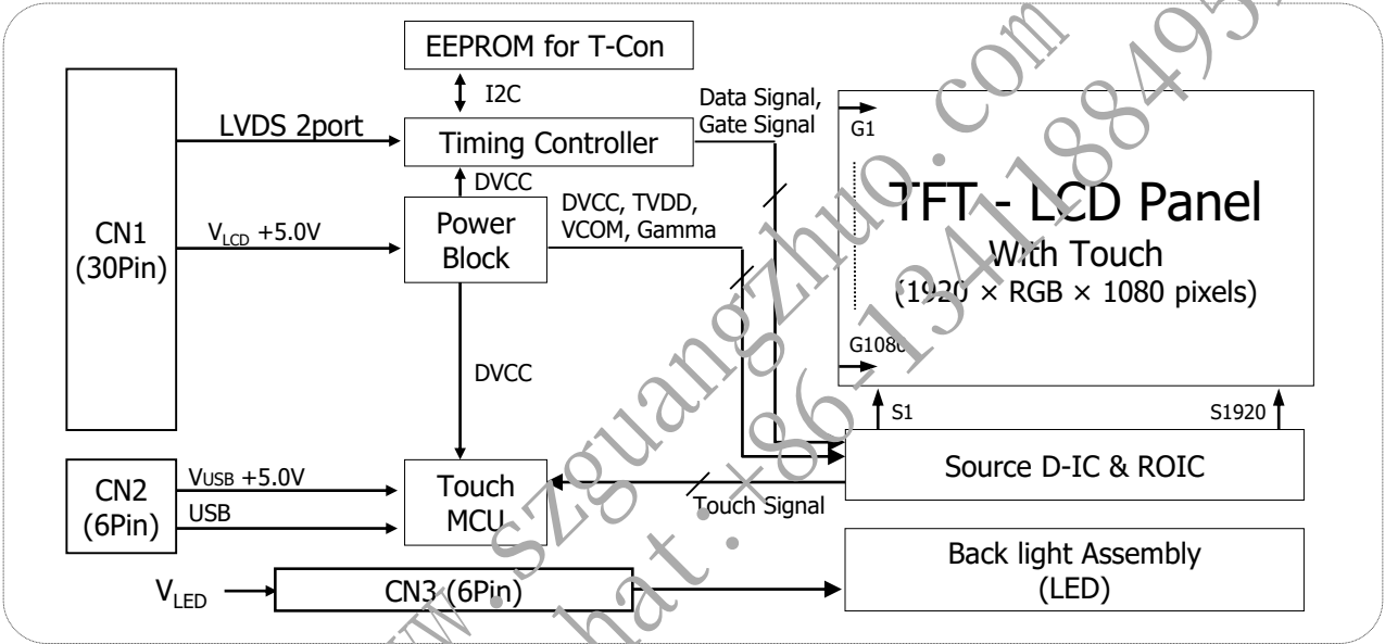
FIG.1 Block Diagram
